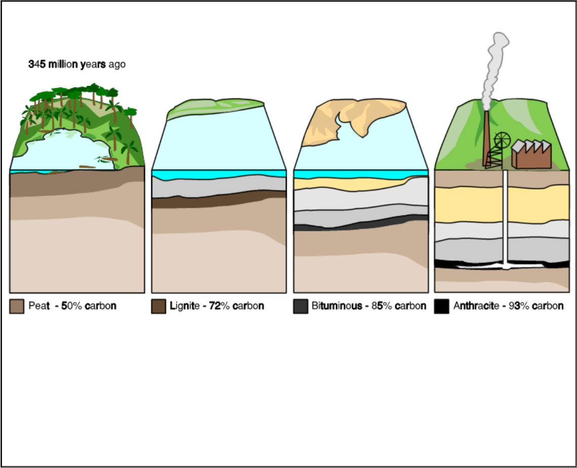
Coal formation
