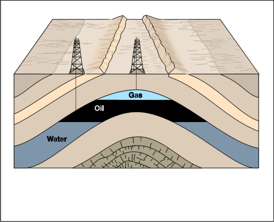
Oil deposit
