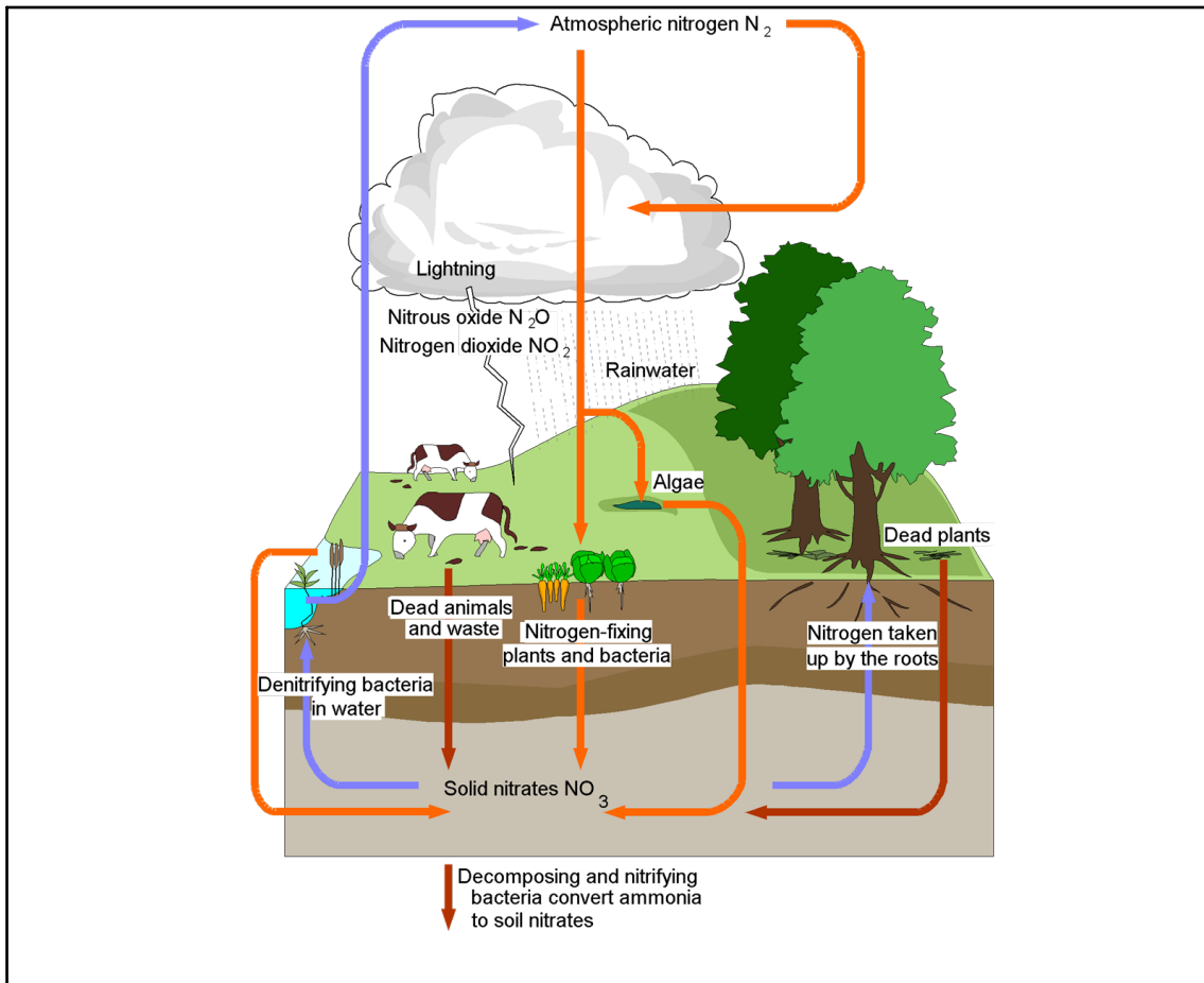
Nitrogen cycle
