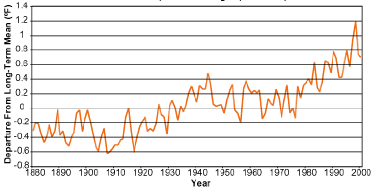
Global Temperature Changes (1880-2000)
