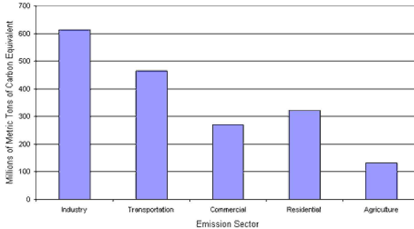
1997 U.S. Greenhouse Gas Emissions by Sector
